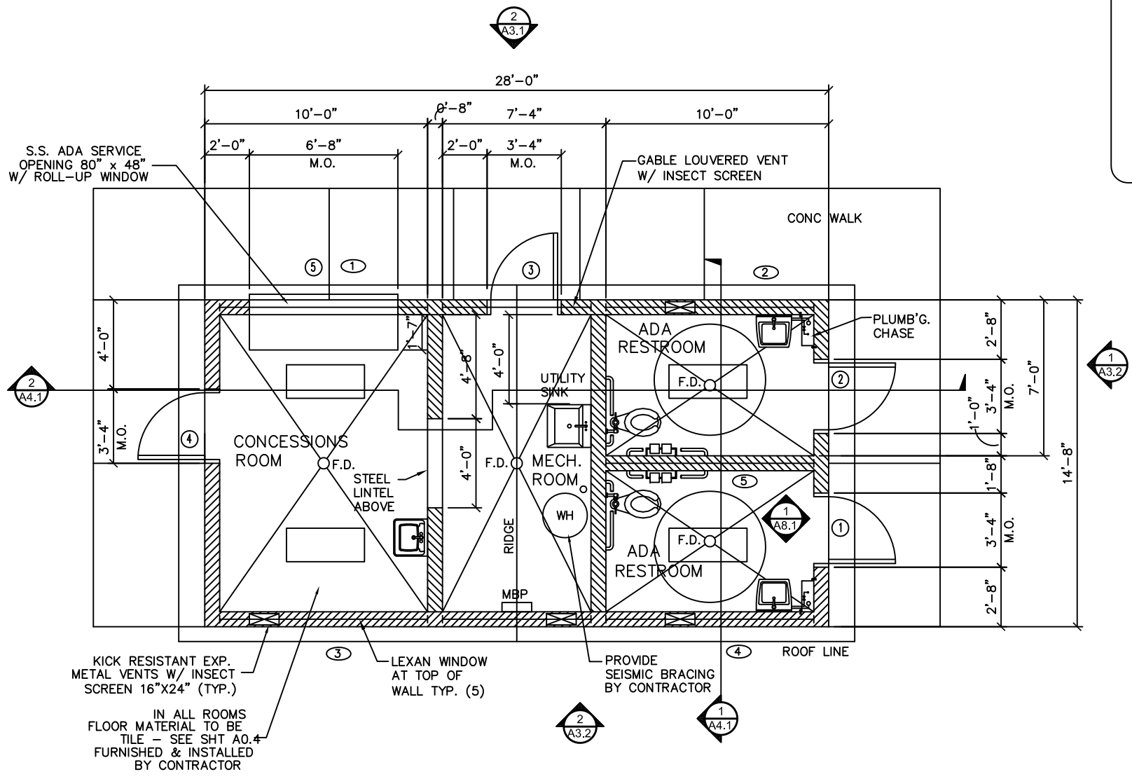
1 FLOOR PLAN SCALE: 1/4" = 1'-0" PLAN NORTH
