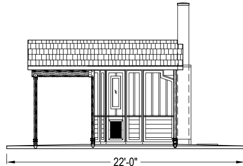
SIDE ELEVATION
