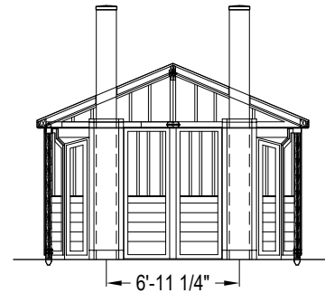
BACK ELEVATION
