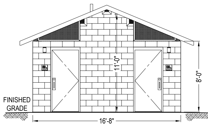
FRONT ELEVATION
