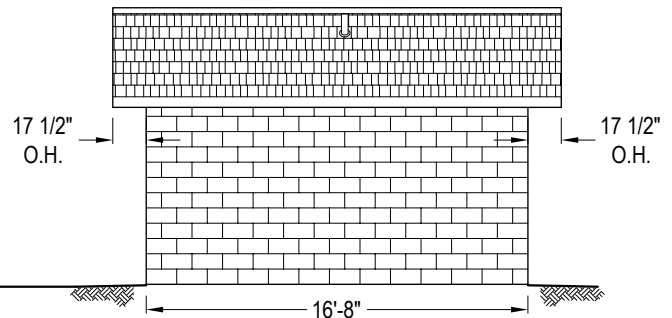
SIDE ELEVATION
