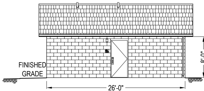
SIDE ELEVATION
