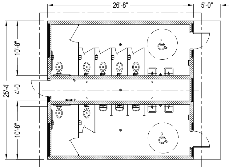
PLAN VIEW
