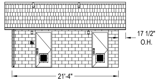
SIDE ELEVATION
