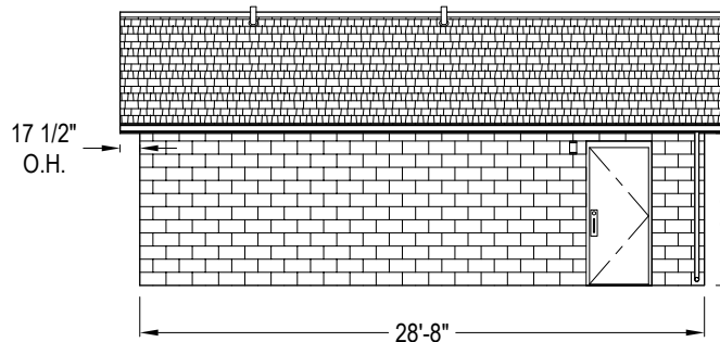
SIDE ELEVATION
