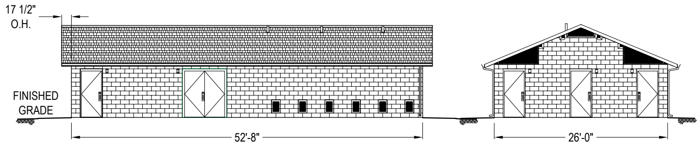
SIDE ELEVATION
