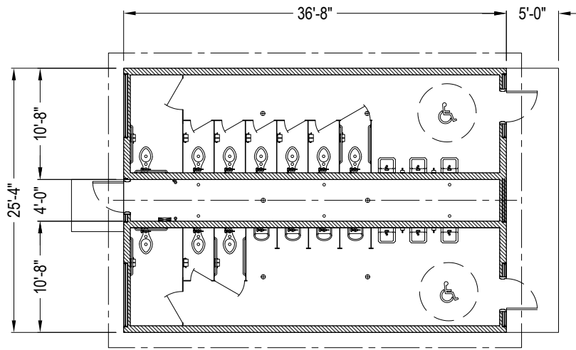
PLAN VIEW
