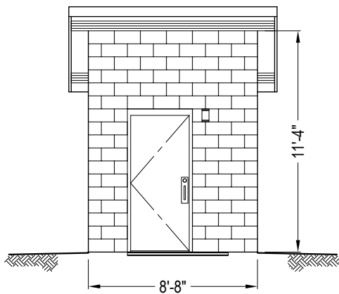
FRONT ELEVATION
