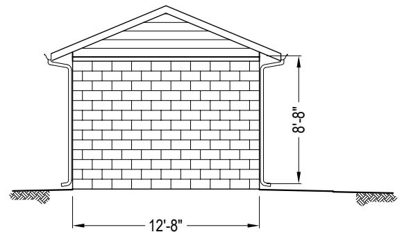
SIDE ELEVATION
