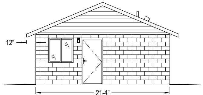
FRONT ELEVATION
