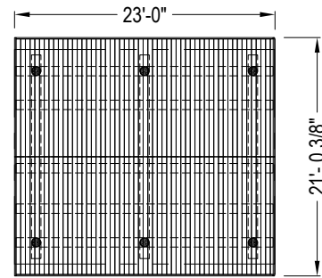
ROOF PLAN VIEW
