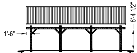
SIDE ELEVATION
