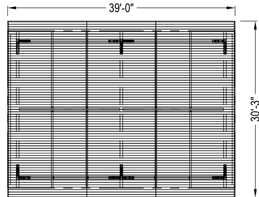
ROOF PLAN VIEW
