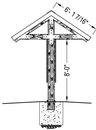
SIDE ELEVATION
