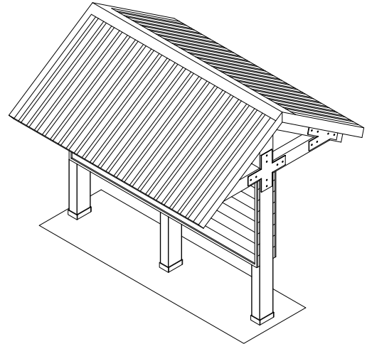
PERSPECTIVE
