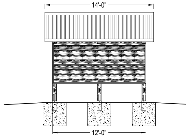
FRONT ELEVATION
