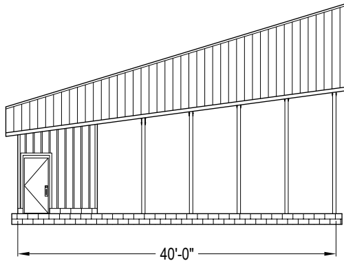
SIDE ELEVATION
