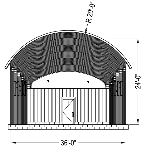
FRONT ELEVATION
